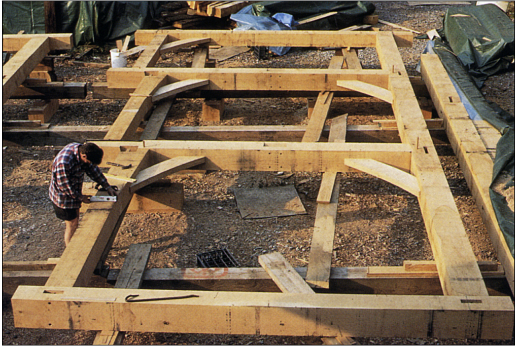
PLATE 8 Frame laid out flat.
